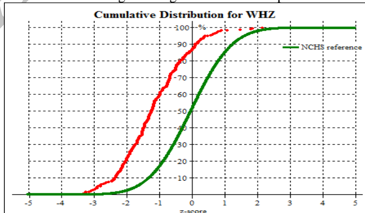
Fig.4: Distribution of weight-for-height z-scores in comparison with standard
