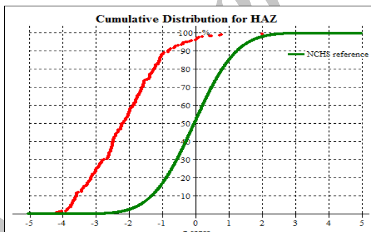
Fig.3: Distribution of height-for-age z-scores in comparison with standard
