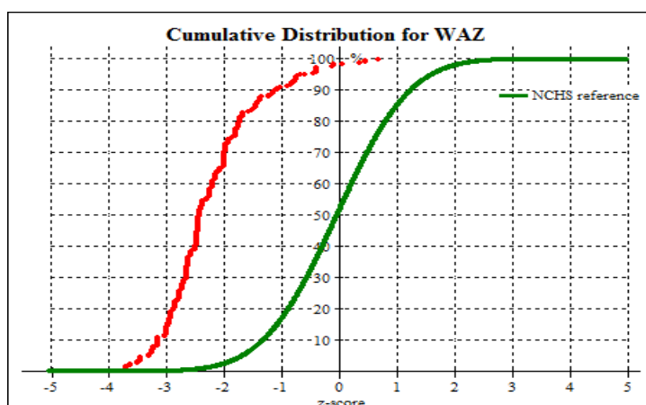
Fig.2: Distribution of weight-for-age z-scores in comparison with standard
