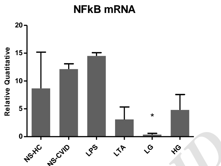
Fig.3: The effect of G2013 on the gene expression of NFκB in CVID patients.
