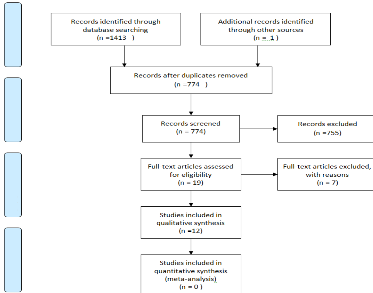
Fig.1: PRISMA flowchart of study.
