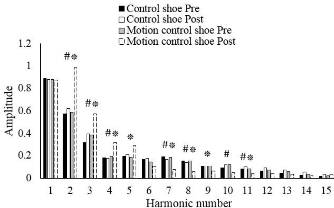
Figure 3. Amplitude versus harmonic number plot of the anterior-posterior ground reaction force. # Significant difference between the control shoes and the motion control shoes testing groups during post-test. * Significant difference between the pre and post-fatigue conditions of the motion control shoes testing condition.
