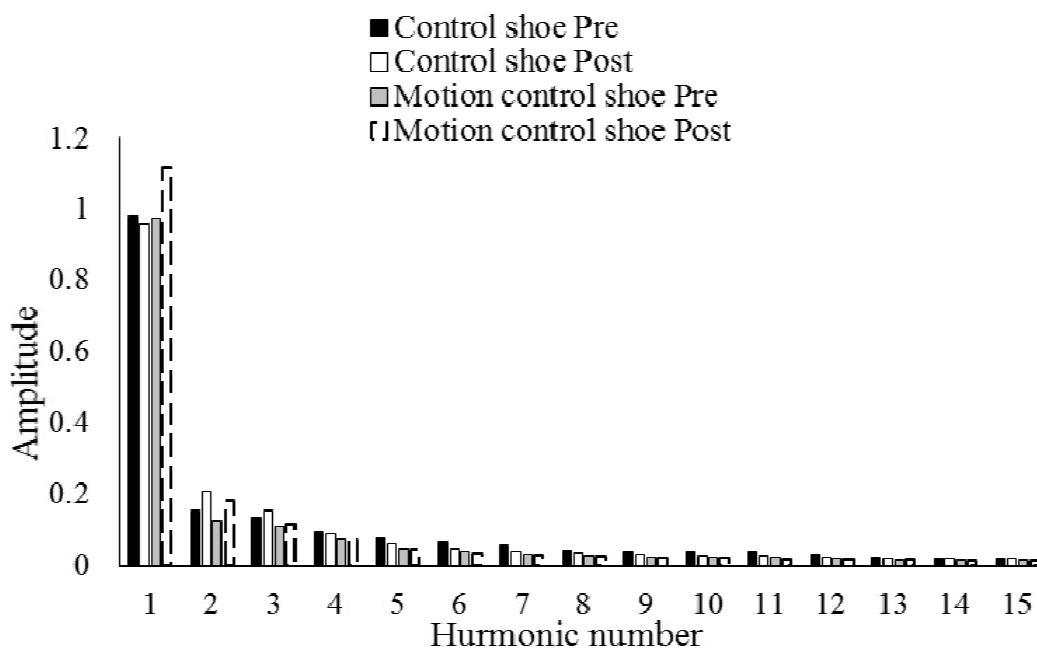
Figure 5. Amplitude versus harmonic number plot of the ( Cop_x ) ground reaction force.
