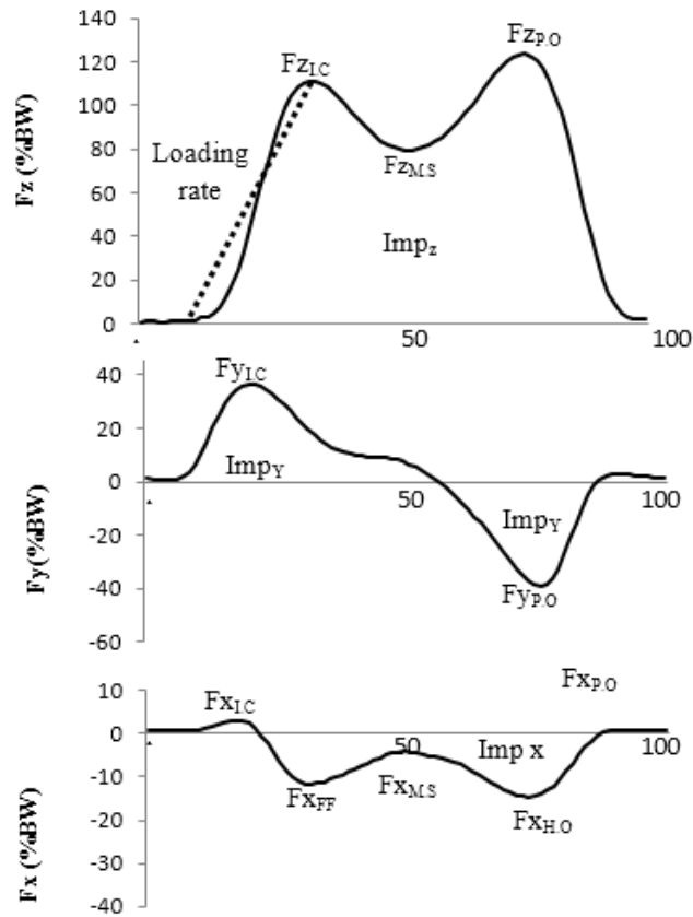
Fig 2: Three dimensional GRF data during walking (20)
