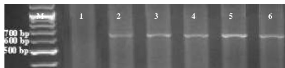
Fig. 3. PCR products (631 bp) obtained with specific primer pairs SUB1/22 from five isolates of F. subglutinans . Lane M: GeneRuler DNA Ladder Mix, 100 to 10,000 bp. 1 = F. proliferatum , 2 = FFSC razi18 weed, 3 = FFSC razi19 weed, 4 = FFSC razi20 weed, 5 = FFSC razi21 weed, 6 = FFSC razi22 weed.
