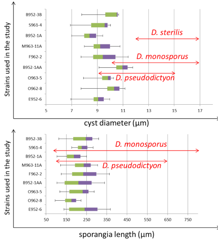
Fig. 2. Boxplots representation of cyst diameter (µm) range (up) and sporangia length (µm) (bottom) of Dictyuchus sp. isolates inferred from 30 measurements of each character. The measurements have been compared to Dictyuchus monosporus , D. pseudodictyon and D. sterilis (when available).
