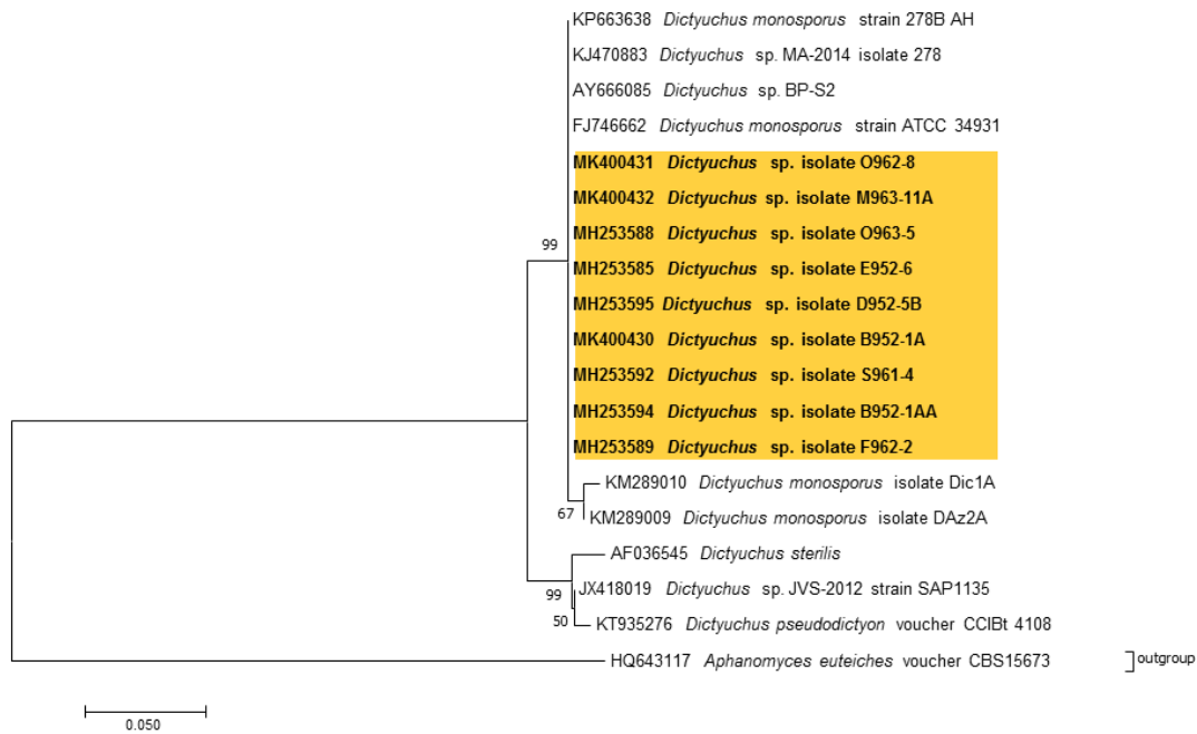
Fig. 3. Molecular phylogenetic tree of the Dictyuchus isolates ( Saprolegniales , Oomycota ). The analysis was performed on alignment of the ITS1-5.8S-ITS2 region of nuclea rDNA (610 bp) using the maximum likelihood method. Numbers next to the branches shows the bootstraps values \geq 50\% . HQ643117 Aphanomyces euteiches was considered as outgroup.
