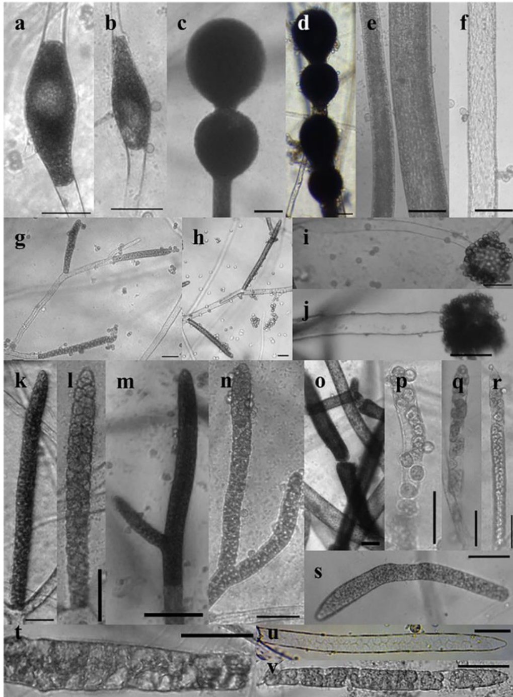
Fig. 1. Morphological structures of Dictyuchus sp. isolates: a–b. fusiform, intercalary gemma; c–d. spherical, terminal, catenulate gemma; e–f. dark (e) and hyaline (f) slender hyphae; g–h. sympodial renewal of fusiform sporangia, usually with only two successions; i–j. achlyoid discharge mode of zoospores four days after inoculation in water culture; k. immature fusiform sporangia; l. mature sporangia before dictyoid discharge; m–n. immature (m) and mature branched sporangia; o. segmentation of hyphae in one month water culture; p–r, t–v. dictyoid discharge mode of zoospores 10 days after inoculation in water culture in different stage of disintegration; (s) curved and detached immature sporangia. — Scale bars = 50 μm.
