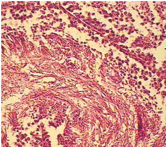
Figure 1. Photomicrograph of FUNAAB-alpha (450 \mu\text{m} ) testis showing normal features with lots of spermatozoa in the seminiferous tubules.
