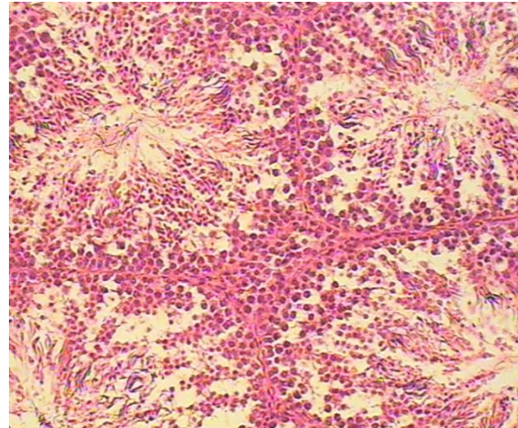
Figure 3. Photomicrograph of a Bantam (450 \mu\text{m} ) testis showing normal seminiferous tubules with normal spermatogenic cell series.
