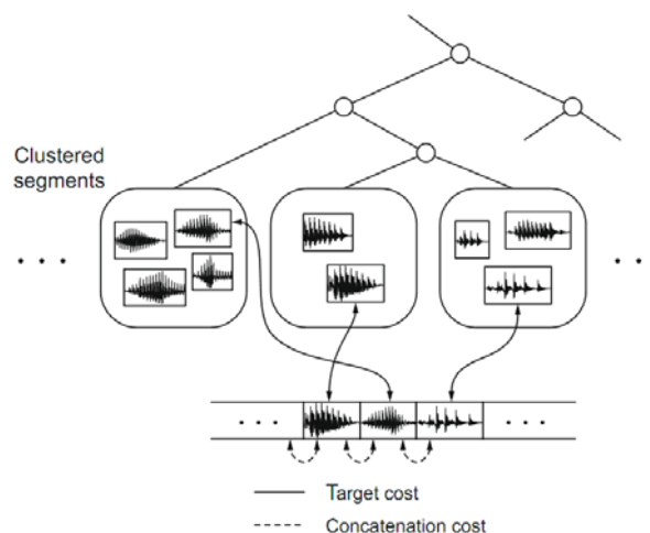
Fig. 2. General Scheme of Clustering in the Unit-Selection Speech Synthesis [3]
