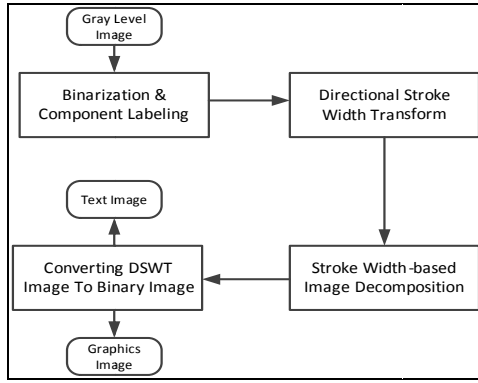
Fig. 1. Block diagram of text/graphics separation.
