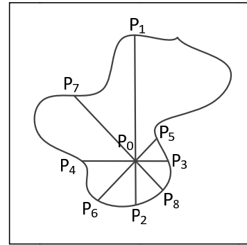
Fig. 3. A Connected Component C , P_1P_2 is vertical line segment, P_3P_4 is in horizontal and P_5P_6 is in diagonal 45 degrees and P_7P_8 is in diagonal 135 degrees. Euclidian Distance between P_{2i-1} and P_{2i} passing through P_0 is calculated for i = 1 to 4. DSWT in P_0 is the smallest length of P_{2i-1}P_{2i} in four orientations, DSWT is the value of stroke width in corresponding point. In this figure, the length of P_5P_6 is the corresponding stroke width of P_0 .
