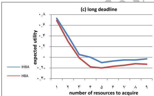
Fig. 7. The number of resources and expected utility (a:short; b:moderate; c:long)
