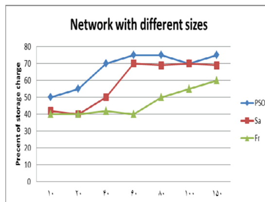
Fig. 4. The rate of final cost optimization with different network size.
