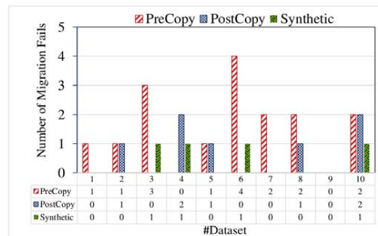
Figure 7: VM live migration fails in the three methods
