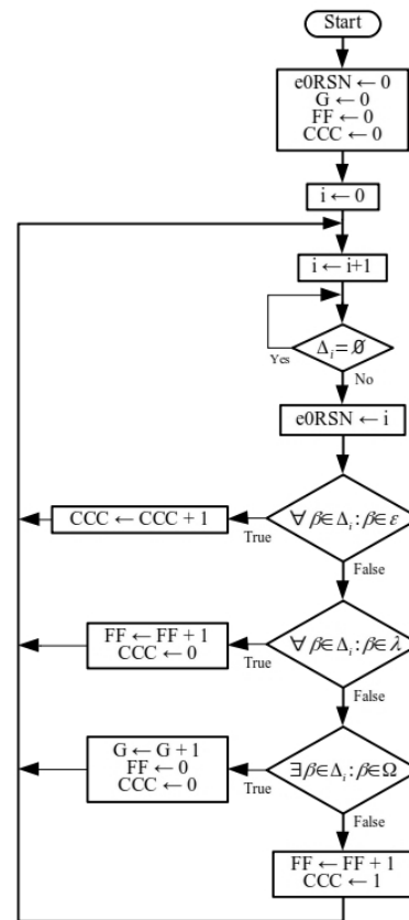
Figure 2: Algorithm for changing QAVNS fields
