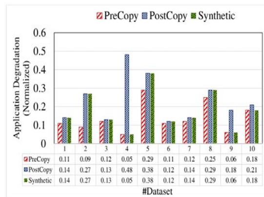
Figure 4: Average performance degradation of applications in PreCopy, PostCopy & proposed methods
