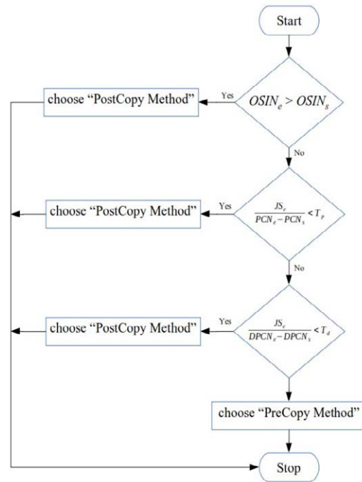
Figure 3: Our decision making algorithm based on QAVNS fields values
