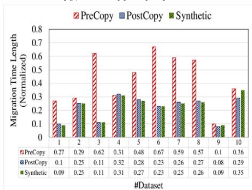
Figure 6: Average time length of virtual machine migration in PreCopy, PostCopy & proposed methods
