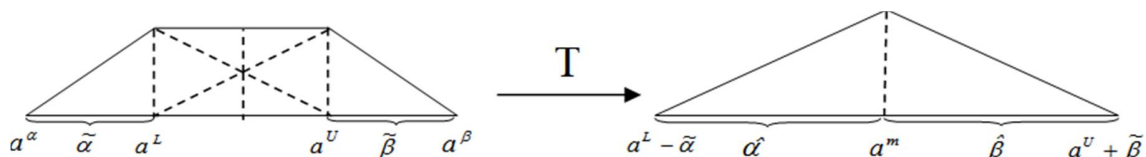
Fig 3. A transformation of the trapezoidal fuzzy number to the triangular fuzzy number
