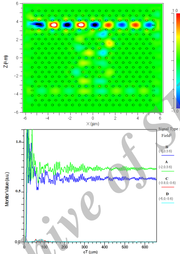
Fig. 5. a) Schematic of pulse propagation in the proposed structure in \lambda=1.2 \mu\text{m} , b) schematic of transmitted powers in different ports.
