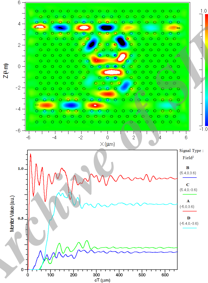
Fig. 3. a) schematic of pulse propagation in the proposed structure in \lambda=1.55\mu\text{m} , b) schematic of transmitted powers in different ports
