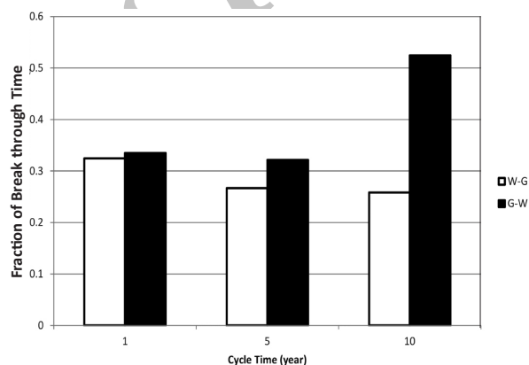
Figure 8: FBT comparison at several cycle times for two conditions, namely W-G and G-W in water wet rock.
