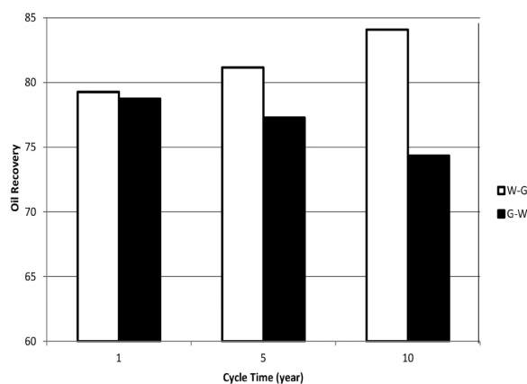
Figure 7: Recovery comparison for several cycle times for two conditions, namely W-G and G-W in water wet rock.
