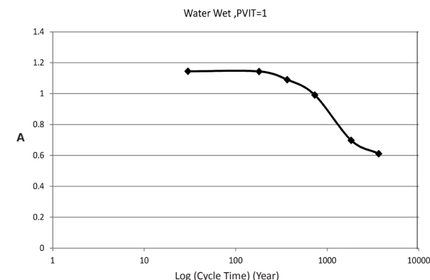
Figure 6: A value (recovery from economical view) at different cycle times in water-wet rock (PVIT=1).
