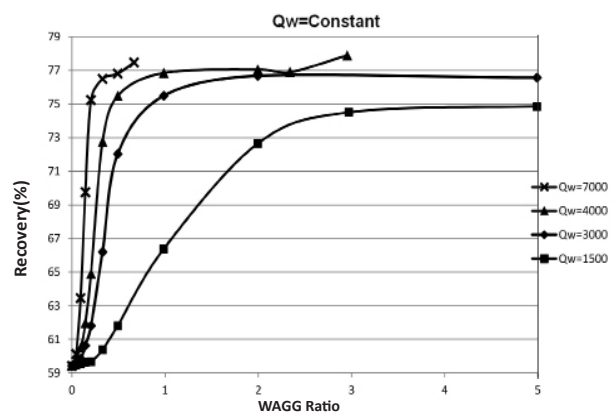
Figure 9: Recovery at different WAGG ratios; water rate is kept constant for each curve.
