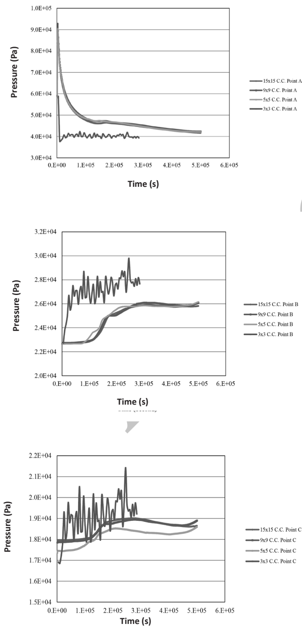
Figure 9: Pressure history at points A, B, and C through different mesh sizes.
