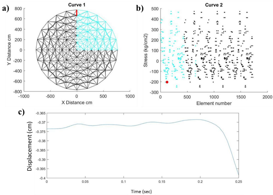
Fig. 4. Vibration of the vertex of the dome after removal of member 123: a) location of the removed element, b) stress level at removed element, c) Vibration of the vertex of the dome
