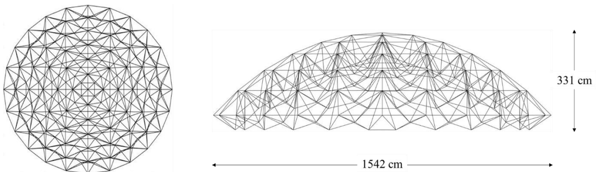
Fig. 1. Dimensional characteristics of the investigated structure
