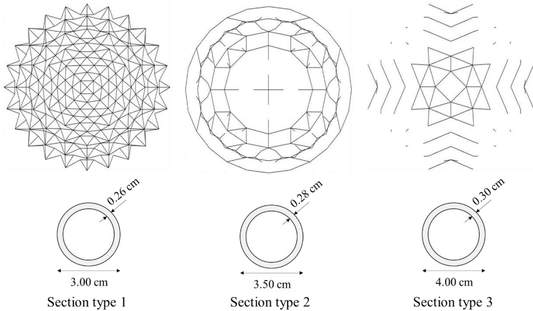
Fig. 2. Section profiles used for structural elements
