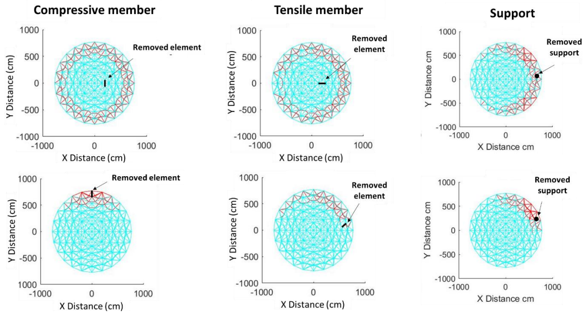
Fig. 6. Pattern of progressive collapse for elimination of compressive members, tensile members and supports
