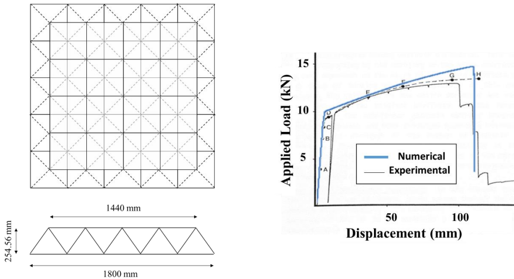
Fig. 3. Structure used for verification and comparison of results
