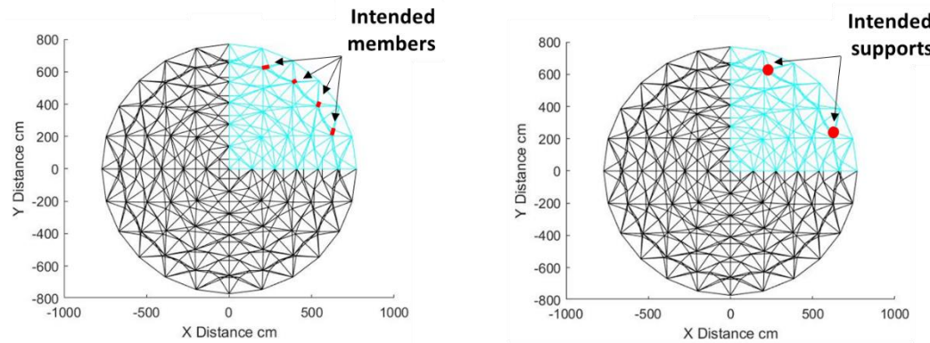
Fig. 5. Members and supports which their elimination cause progressive collapse at 140% of the gravity loads
