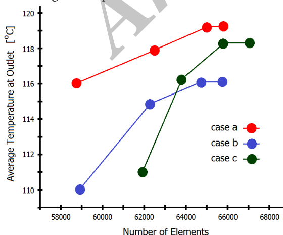
Fig. 3. Grid independency study for the average temperature at outlet.
