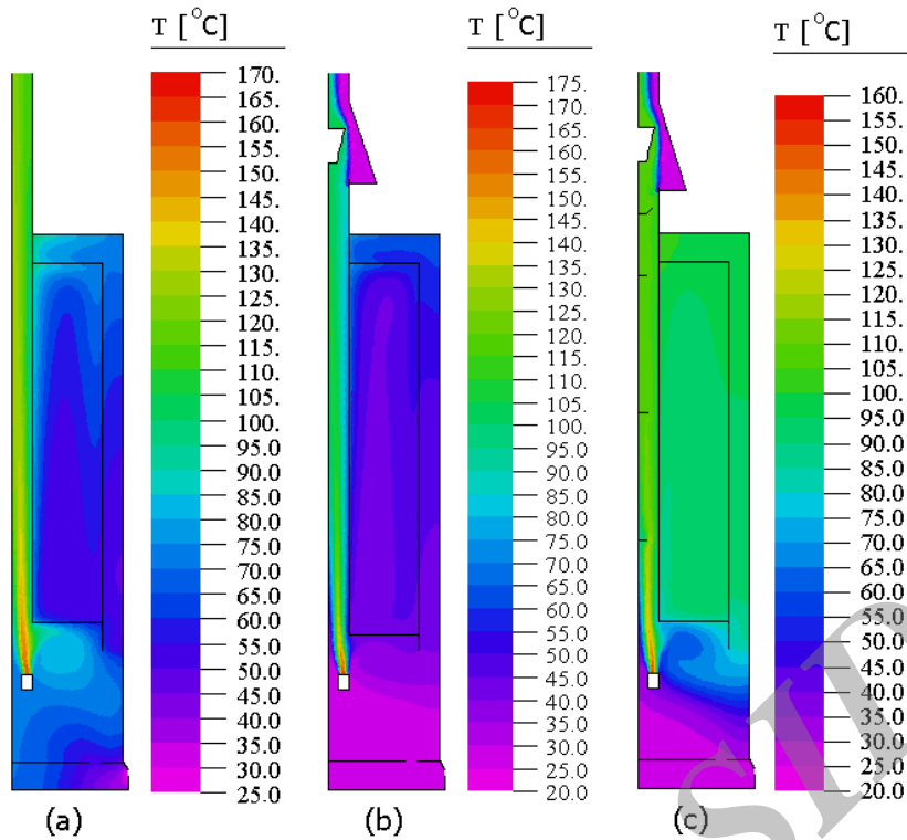
Fig.4. Temperature distribution of the system in three considered cases (a) without vent hood and flue baffles, (b) with vent hood and without flue baffles, and (c) with both vent hood and flue baffles.
