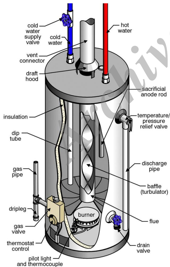
Fig. 1. A schematic view of the gas water-storage heater and its components [16].
