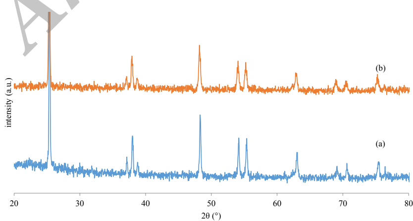
Fig. 3- The XRD patterns of (a) \text{TiO}_2 and (b) \text{TiO}_2/\text{SG} nanocomposites prepared at 700 °C, with a deposition time of 60 min.
