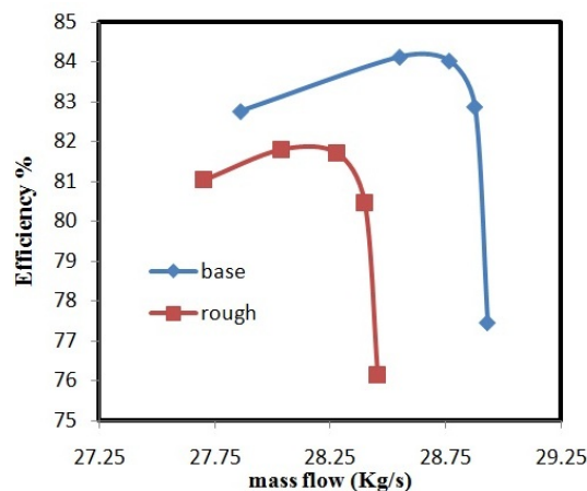
Fig.22. Isentropic Efficiency Vs. the Mass Flow
