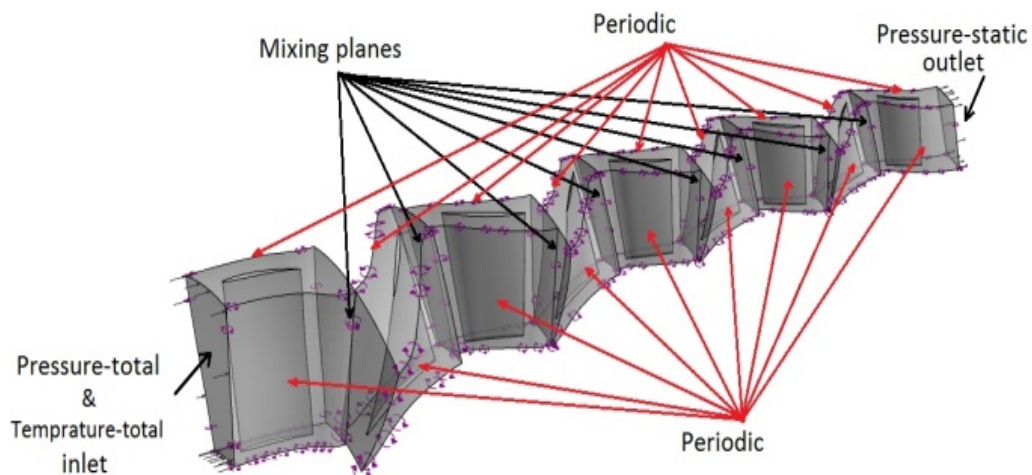
Fig.7. Boundary Conditions used in Simulation
