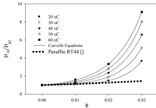
Fig. 5. Relative viscosity versus solid volume fraction for various temperatures and data for paraffin RT44[31]
