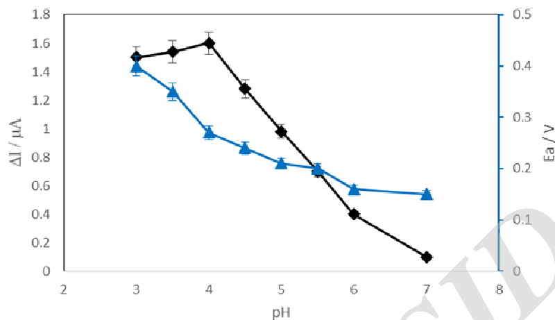
Fig. 5. The effect of pH of the anodic peak current and electrooxidation potential of 0.31 mM of AA, in PBS (pH 4) at scan rate 50 \text{ mV s}^{-1} .
