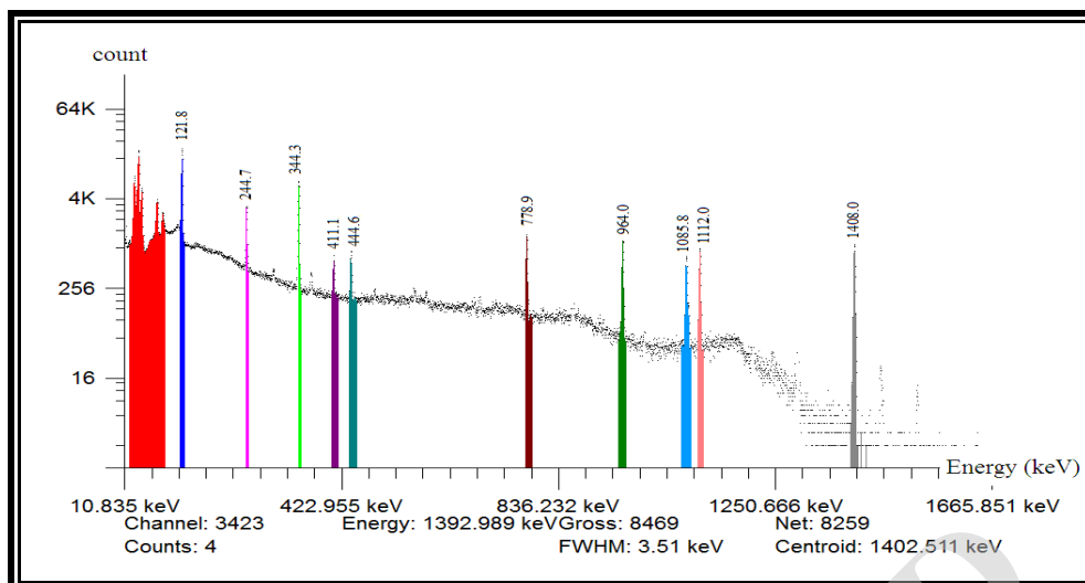
Fig. 2. 152 Eu spectrum of the prepared standard source
