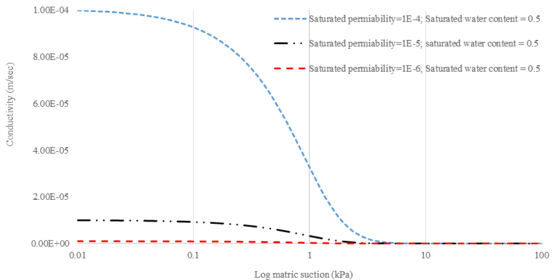
Fig. 5. Matric suction V.S soil conductivity considering different saturated condition
