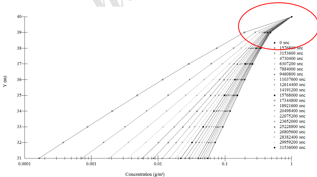
Fig. 9. Values of vertical oil concentration, considering K=1e-6 (m/s) in saturated soil condition
