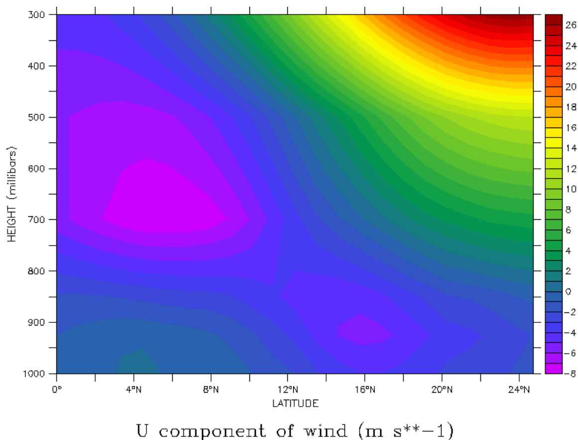
Fig. 7. The vertical cross section of mean zonal wind for winter (November – March). The AEJ is located around 600–750 hpa and the core is centered around 650–700hpa around Latitude 4°N. Low level Jet (LLJ) is also observed at 900 hpa at Latitude 16°N
