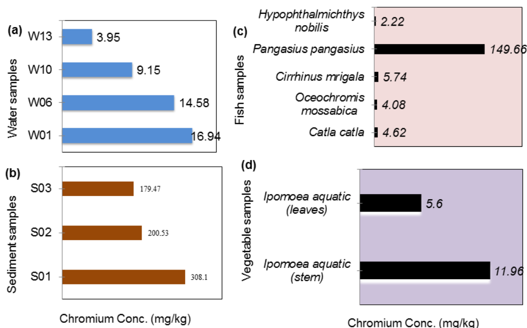
Fig. 3. Concentrations of Chromium (Cr) in Lake (a) water; (b) sediment; (c) fish and (d) vegetable samples.
