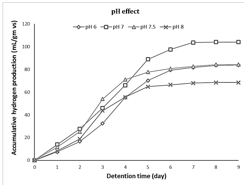
Fig. 2. Accumulative hydrogen production at different pH, TS=10%, Temp. 30°C and mixing ratio = 1:5
