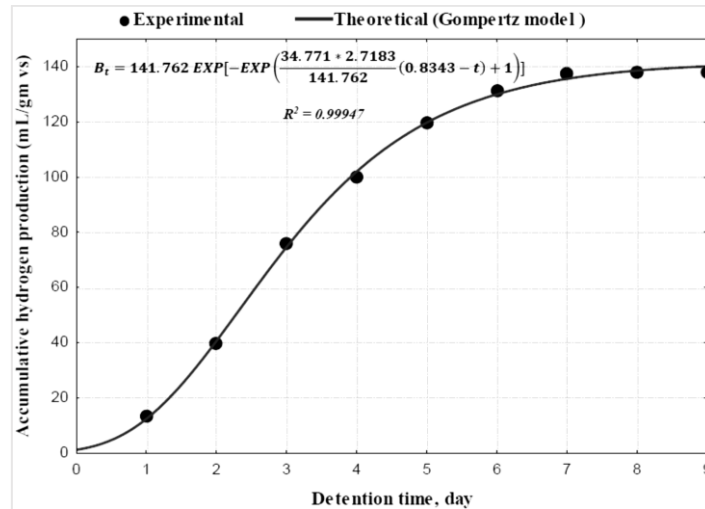
Fig. 13. Examination of experimental data and modified Gompertz model for hydrogen production.
