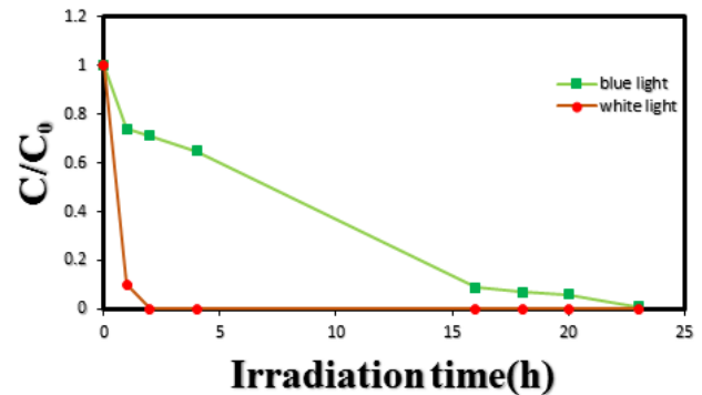
Figure 8. Investigation of the effect of light source on the photocatalytic activity of MWCNT/TiO 2 thin films.
