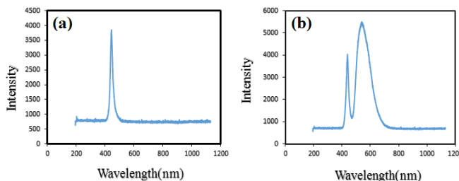
Figure 7. Spectra of two light sources. (a) Blue light (450 nm), (b) White light (450-700nm).
