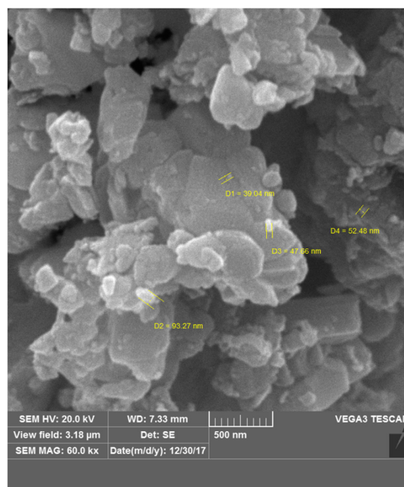
Figure 4- a. SEM image for Nd-1111.
