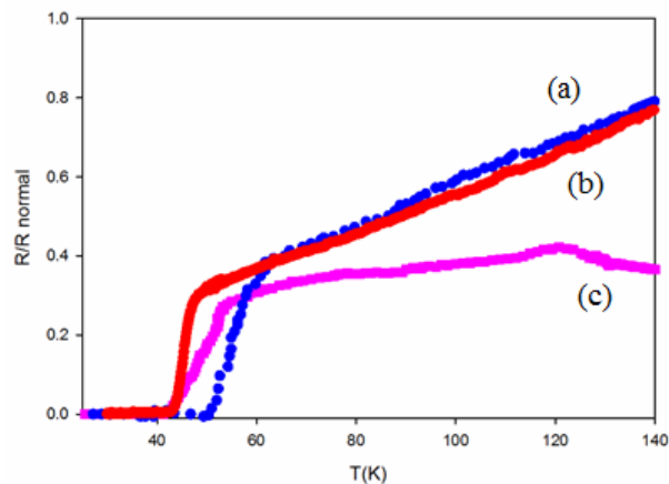
Figure 5. The normalized resistivity of (a) Nd-1111(blue line), (b) Nd-Sb0.05(red line) and (c) Nd-Ca0.01 (pink line).
