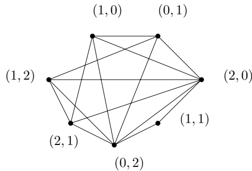
FIGURE 2. The graph \Gamma_0(\mathbb{Z}_{36}) .
