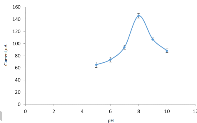
Fig. 4. Dependence of the oxidation peak current of 1 \times 10^{-3} M QR on pH values in 0.1 M PBS buffer, at a scan rate of 100 \text{ mVs}^{-1}
