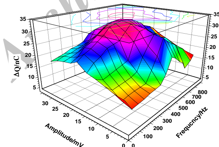
Fig. 4. The effect of frequency and amplitude on the response of DNA-AuNPs/MWCNT-IL/GCE for solution of 8 nM of TM
