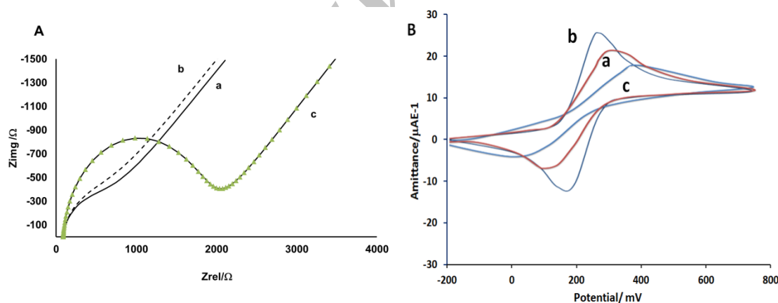
Fig. 2. A) EIS plots of modified electrode in 3 mM \text{K}_3\text{Fe}(\text{CN})_6 with : (a) bare GCE, (b) AuNPs/MWCNT-IL/GCE and (c) DNA-AuNPs/MWCNT-IL/GCE. and B) Cyclic voltammograms of 3 mM \text{K}_3\text{Fe}(\text{CN})_6 in buffer on (a) bare GCE, (b) AuNPs/MWCNT-IL/GCE and (c) DNA-AuNPs/MWCNT-IL/GCE
