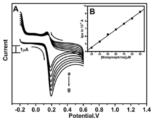
Fig. 6. (A) Cyclic voltammograms of NE in 0.2 M PBS solution of pH 7.4 at poly(CR) MCPE at scan rate of 100 \text{ mVs}^{-1} with different concentrations (a–g: 30 \mu\text{M} , 40 \mu\text{M} , 50 \mu\text{M} , 60 \mu\text{M} , 70 \mu\text{M} , 80 \mu\text{M} , 90 \mu\text{M} ); (B) Graph of anodic peak current versus concentration of NE
