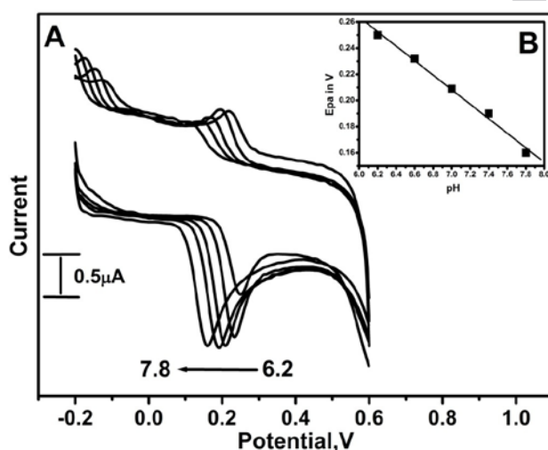
Fig. 7. (A) Cyclic voltammograms of the poly (CR) MCPE in 0.2 M PBS solution at different pH values (a–e: 6.2 to 7.8) at scan rate of 100 mV/s; (B) Graph of the anodic peak potential versus pH
