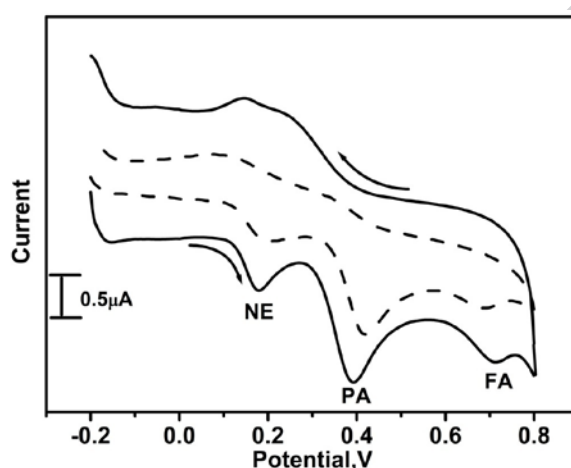
Fig. 8. Cyclic voltammograms for simultaneous determination of 0.3 mM NE, 0.1 mM PA and 0.1 mM FA in 0.2 M PBS (pH 7.0) at BCPE (dashed line) and poly (CR) MCPE (solid line) at scan rate of 100 mV/s
