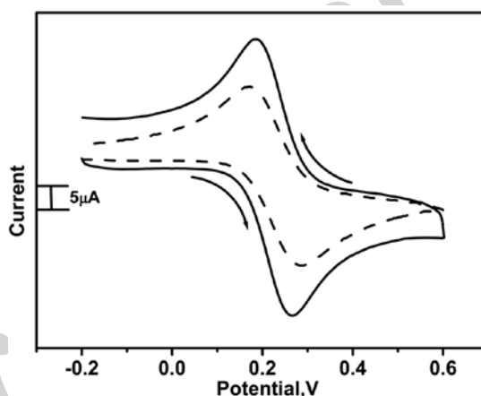
Fig. 3. Cyclic voltammograms of 1 mM potassium ferrocyanide at BCPE (dashed line) and poly (CR) MCPE (solid line) at scan rate of 50 mV/s
