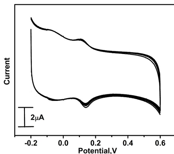
Fig. 12. Cyclic voltammograms for 10 multiple cycles of 0.3 mM NE in 0.2 M phosphate buffer solution pH 7.4 at Poly (CR) MCPE at the sweep rate of 100 mV/s
