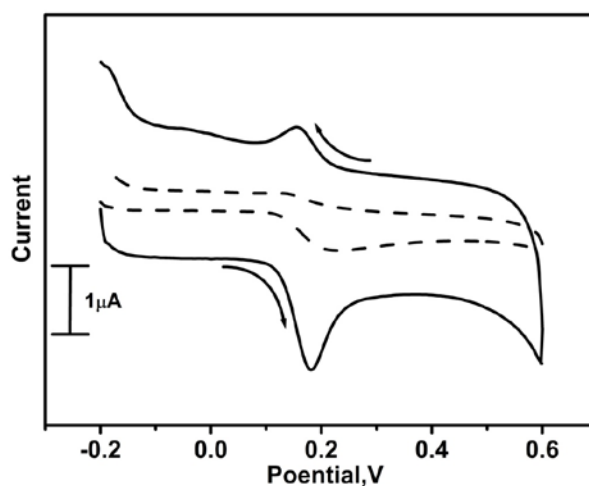
Fig. 4. Cyclic voltammograms of 0.3 mM NE in 0.2 M PBS solution of pH 7.4 at BCPE (dashed line) and poly (CR) MCPE (Solid line) at scan rate of 100 mV/s
