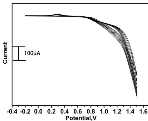
Fig. 1. Electropolymerization of 0.5 mM of Congo red at 0.1 M NaOH as supporting electrolyte for 10 cycles with Sweep rate of 100 mV/s
