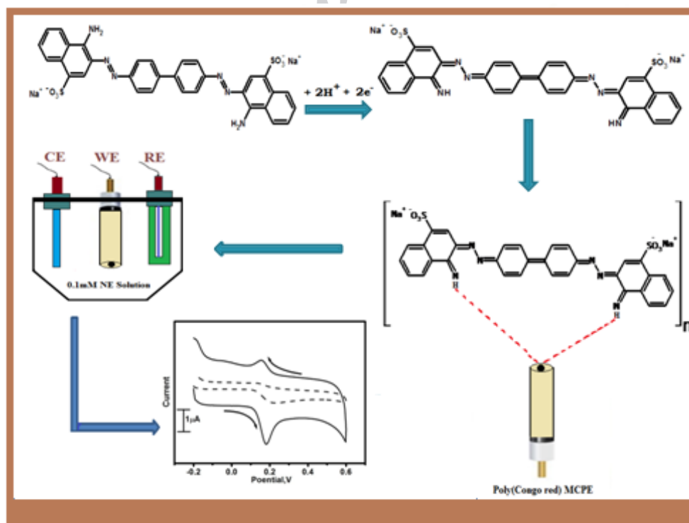
Scheme 1. The detailed oxidation mechanism of Norepinephrine
