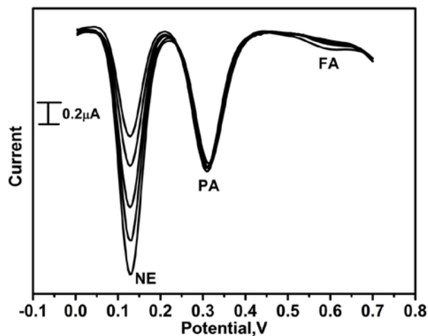
Fig. 9. Differential pulse voltammogram recordings for varying concentration of NE (a-e: 0.1-0.5 mM) in presence of constant 0.2 mM PA and 0.2 mM FA at poly (CR) MCPE
