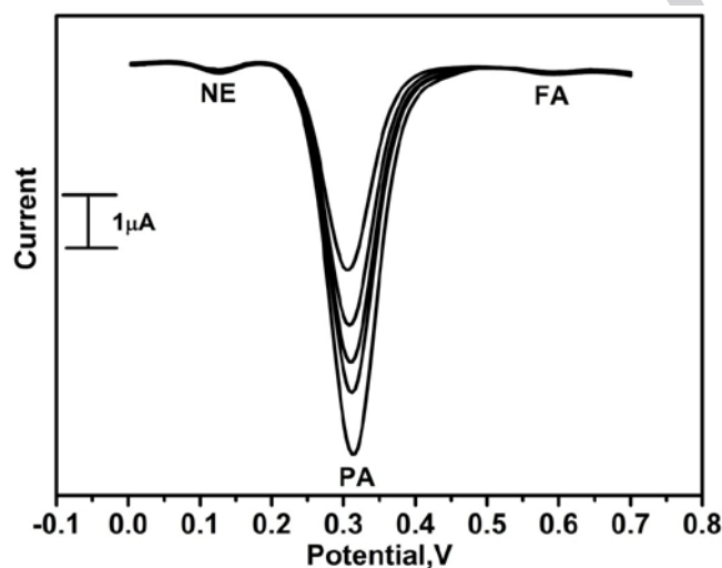
Fig. 10. Differential pulse voltammogram recordings for varying concentration of PA (a-e: 0.1-0.5 mM) in presence of constant 0.2 mM NE and 0.2 mM FA at poly (CR) MCPE
