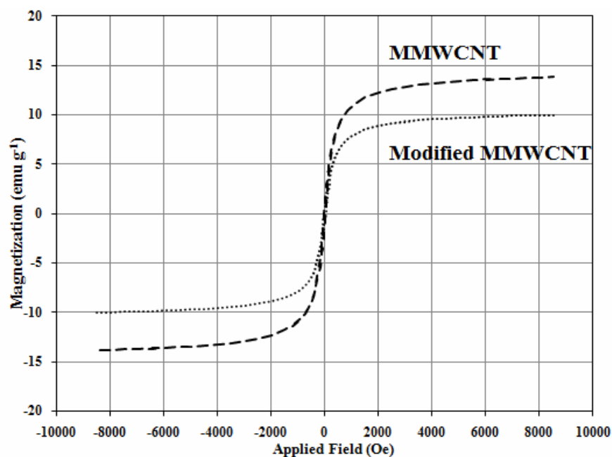
Fig. 5. Magnetic hysteresis curves of MMWCNT and modified MMWCNT.
