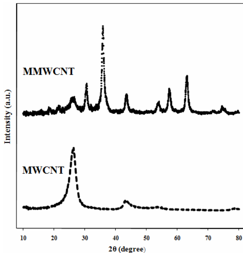
Fig. 2. XRD patterns of MWCNT and magnetic MWCNT (MMWCNT) nanocomposite.
