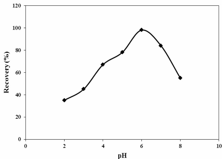
Fig. 6. The effect of sample solution pH.
