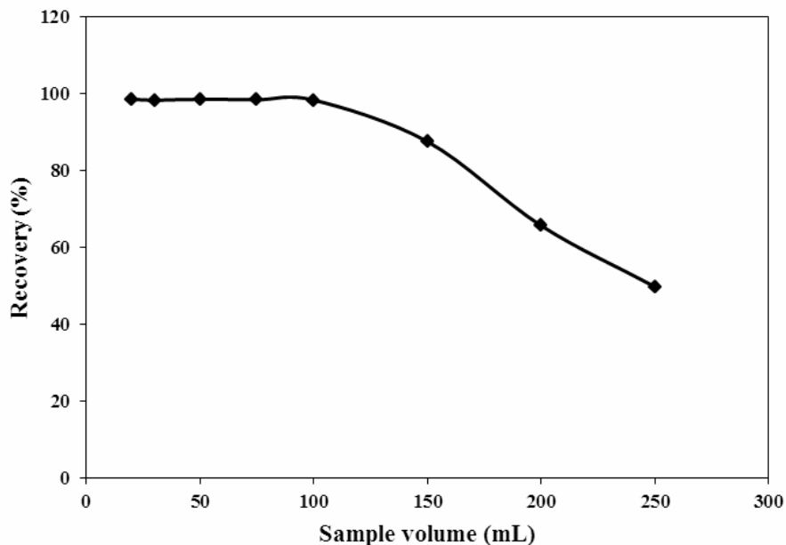
Fig.7. Effect of sample volume on the recovery of Tl(I).
