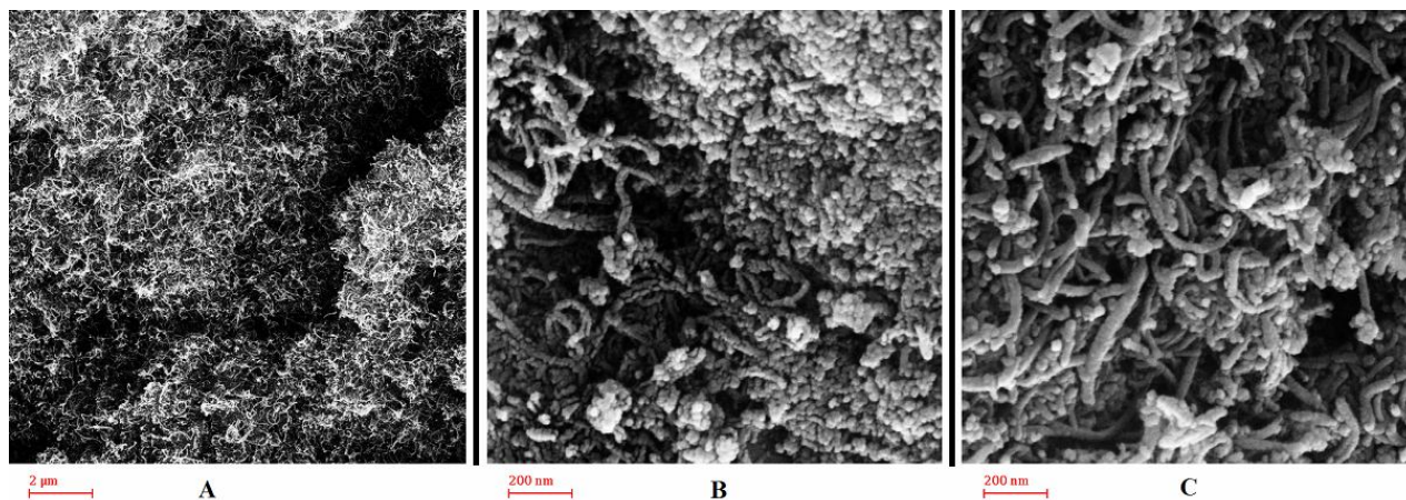
Fig. 4. FE-SEM images of (A) MWCNT, (B) MMWCNT and (C) modified MMWCNT nanocomposite.
