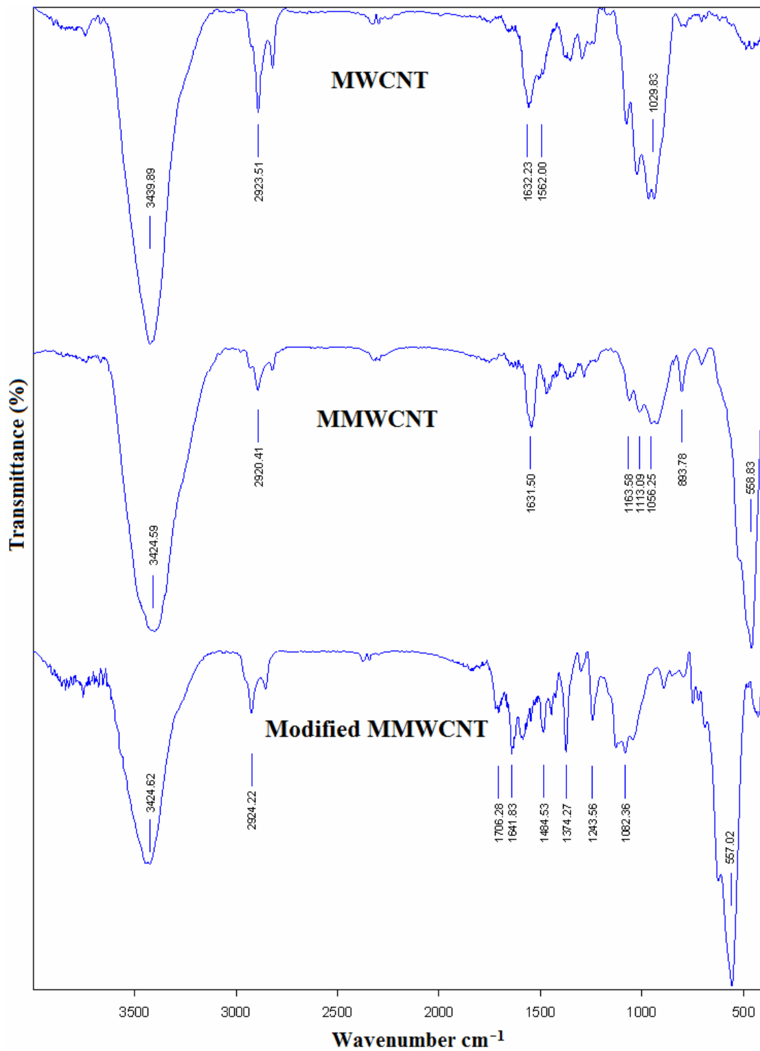
Fig. 3. FT-IR spectra of MWCNT, MMWCNT and modified MMWCNT nanocomposite.
