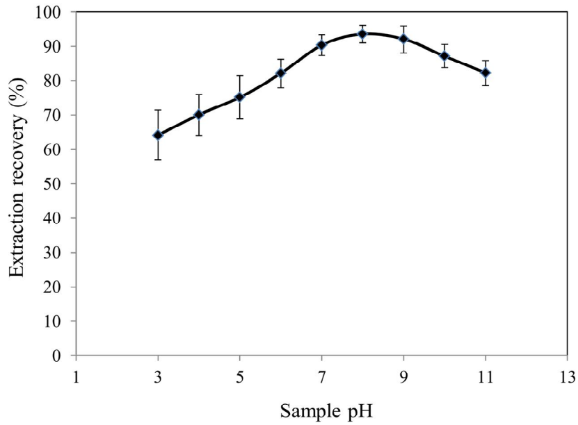
Fig. 1. Effect of the sample pH on the extraction recovery of cadmium. Conditions: cadmium concentration, 10 \text{ ng l}^{-1} ; dithizone concentration, 75 \text{ mg l}^{-1} ; sample volume, 6 ml; extraction solvent, 1-dodecanol ( 30 \text{ } \mu\text{l} ); number of injections, seven times.
