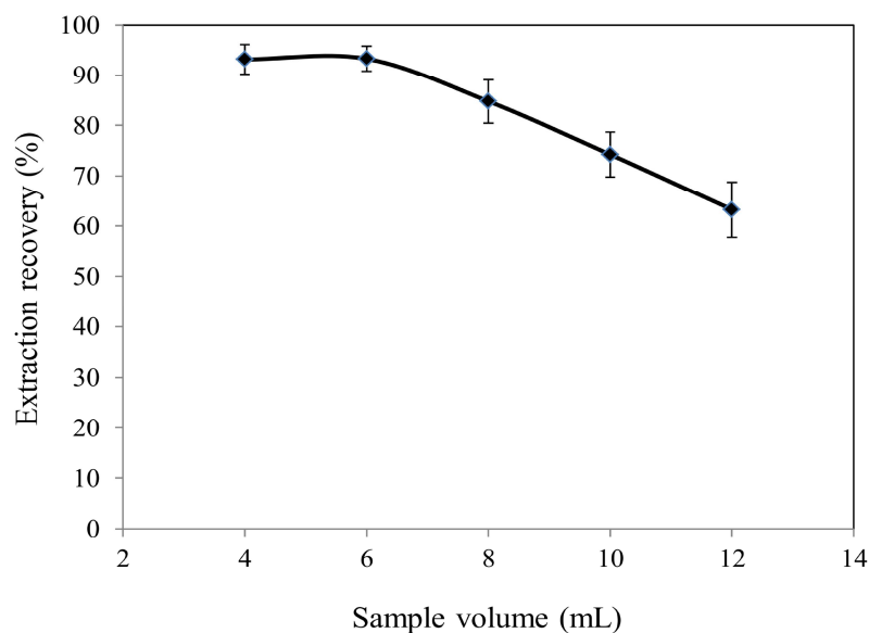
Fig. 3. Effect of the sample volume on the extraction recovery of cadmium. Conditions: sample pH, 8.0; amount of cadmium, 0.06 ng; dithizone concentration, 75 mg l -1 ; extraction solvent, 1-dodecanol (30 µl); number of injections, seven times.
