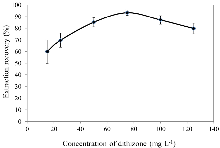
Fig. 2. Effect of the dithizone concentration on the extraction recovery of cadmium. Conditions: cadmium concentration, 10 \text{ ng l}^{-1} ; sample volume, 6 ml; extraction solvent, sample pH, 8.0; 1-dodecanol ( 30 \text{ } \mu\text{l} ); number of injections, seven times.
