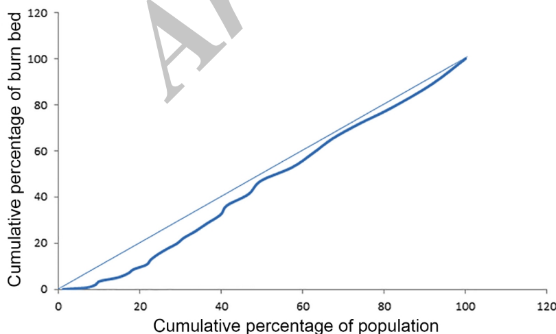
Figure 2. Lorenz curve of burn bed in population level.
