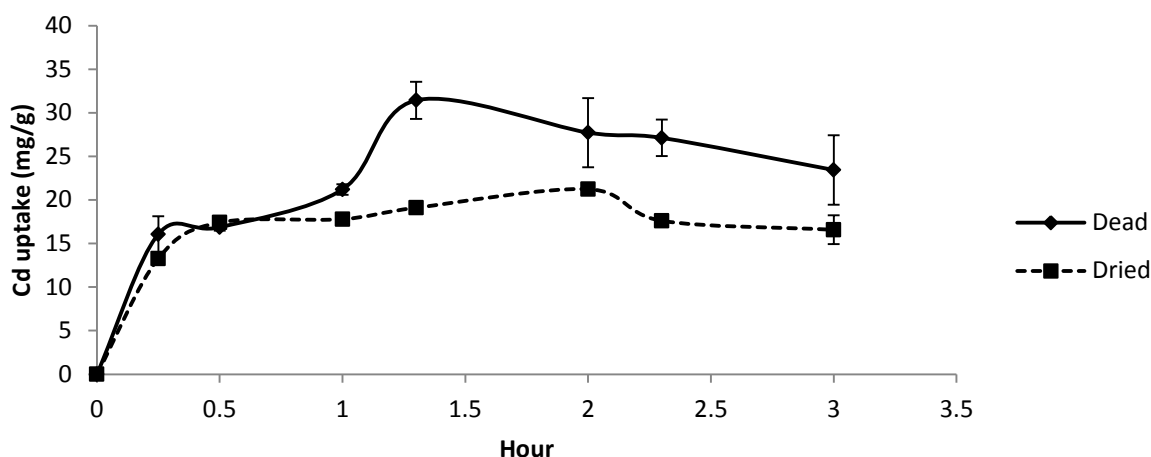
Fig. 2 :Effect of contact time on the Cd removal by dead and dried biomass. Data were found to be significant at P < 0.05 . The vertical line on each bar shows the standard deviation.
