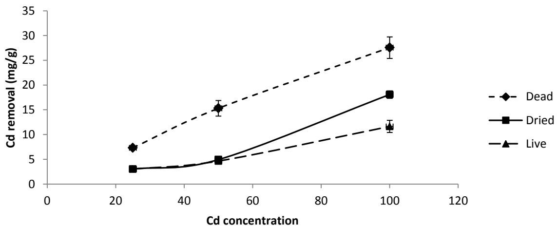
Fig. 4 : Effect of initial Cd concentration on the Cd removal. Contact times of 4 days, 1.30 h and 2 h were performed for live, dead and dried biomass respectively as optimal values. Optimum pH of 4 in case of live and dead biomass and pH of 6 in case of dried biomass were used. Data were found to be significant at P < 0.05 . The vertical line on each bar shows the standard deviation.
