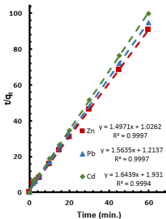
Fig. 9: Pseudo Second Order Models for Removal of Zinc (■), Lead (▲) and Cadmium (◆) ions by Modified Sorbent. Initial Ion Concentration: 100 mg/l, pH: 5, Sample Solution Volume: 500 ml, Sorbent: 15 g, DEHPA in Socking Solution: 0.01 M, Socking Time: 10 h, Shaking Rate: 500rpm, Temperature: 28°C.
