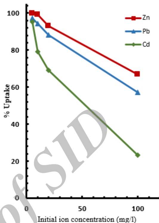
Fig.6: Effect of Initial Concentration on the Sorption of Zinc (■), Lead (▲) and Cadmium (◆) ions on the Modified Sorbent Surface. Sample Solution Volume: 100 ml, pH: 5, Sorbent: 3g, DEHPA in Socking Solution: 0.01 M, Socking Time: 10 h, Temperature: 28°C.
