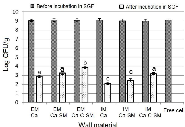
Figure 2: Effect of Microencapsulation on Viability of L. acidophilus in SGF (Ca: calcium-alginate; Ca-SM: mixture of calcium-alginate and skim milk; Ca-C-SM: calcium-alginate coated by skim milk; Superscript letters (a-c) above the error bars that are significantly different [ P < 0.05 ])
