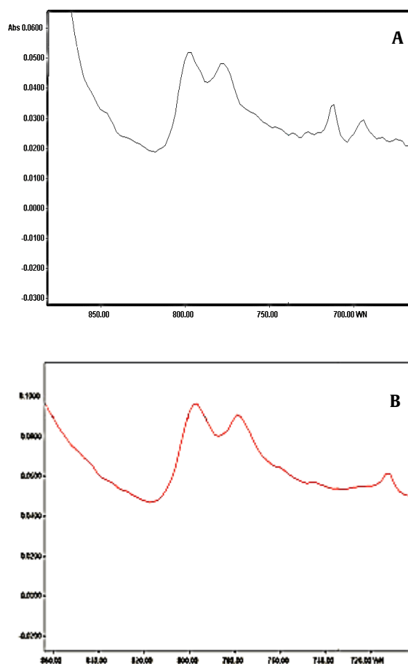
Figure 1: Spectrum Sample of Crystalline Silica Samples of A) Traditional Factories and B) Mechanical Factory Using FT-IR
