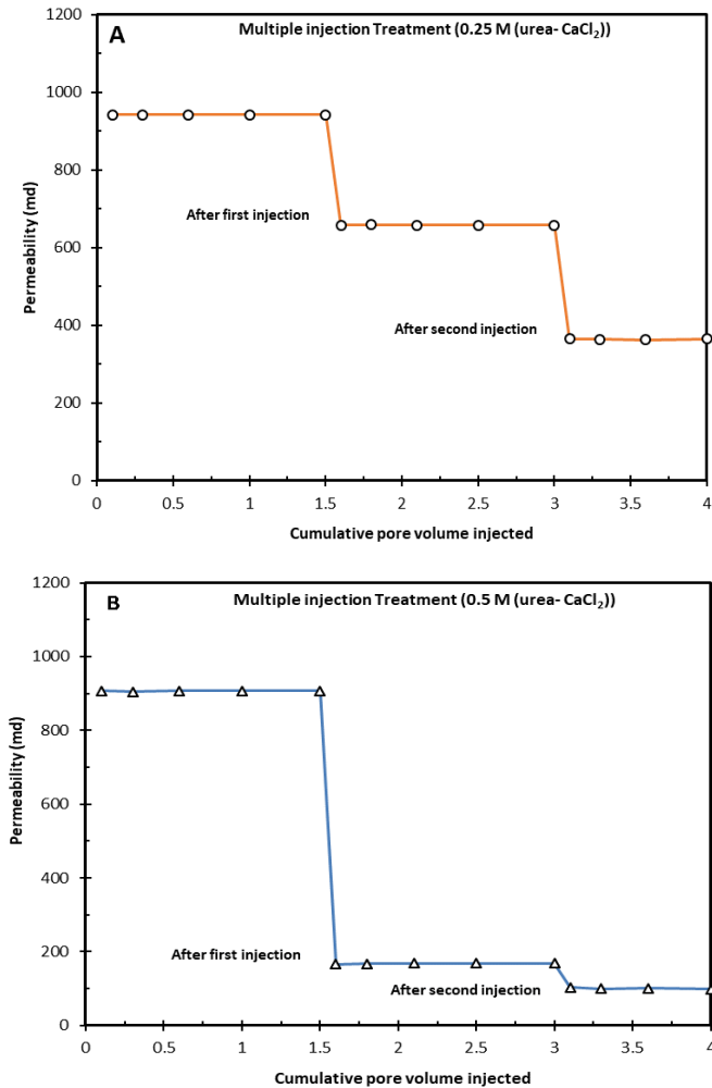
Figure 5: Effect of multistep injection of CS on permeability reduction: CS = 0.25M (A) and CS = 0.5M (B)
