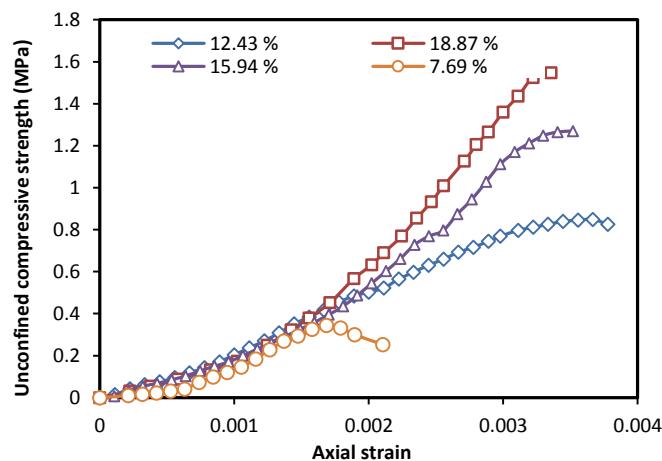
Figure 4: Stress-strain curve of biologically treated soil samples at different CaCO 3 contents
