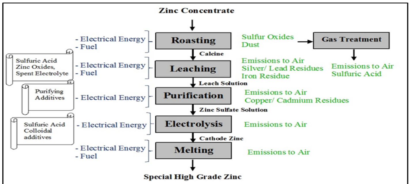
Figure 1: Hydrometallurgical process, energy consumption, and environmental aspects [18]
