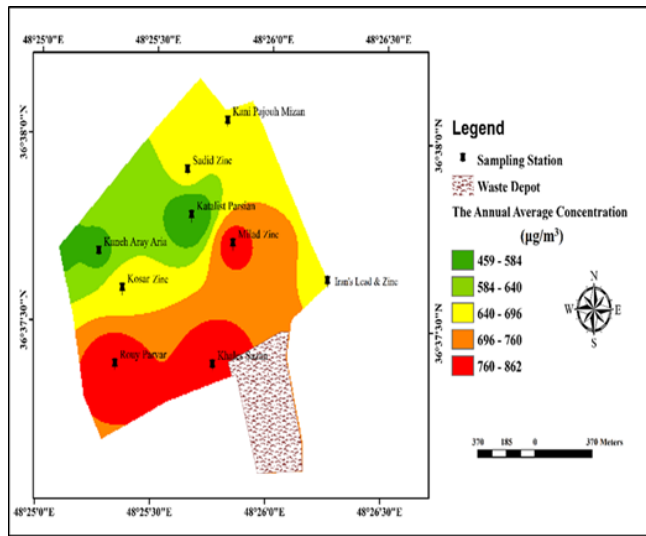
Figure 3: Mean annual concentration of particles in ZZIP
