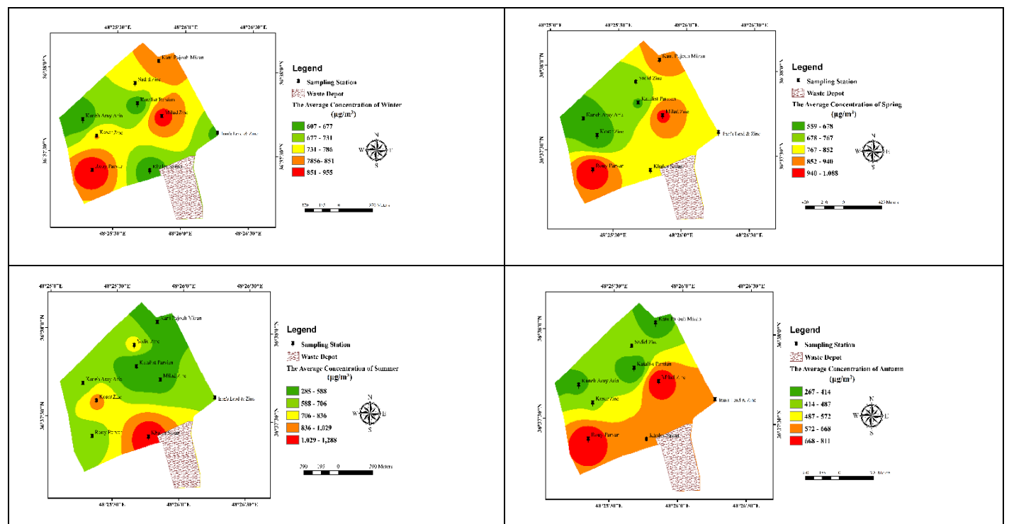
Figure 4: Mean seasonal concentration of particles in ZZIP
