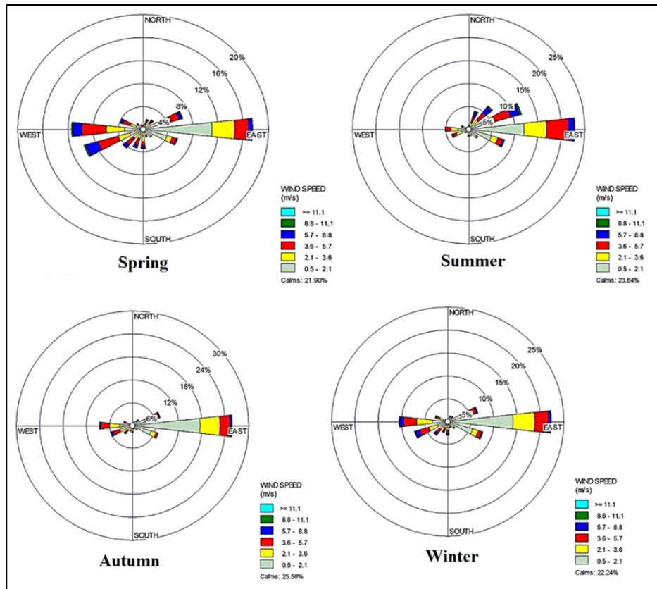
Figure 2: Long-term wind rise changes in different seasons (2008-2018)
