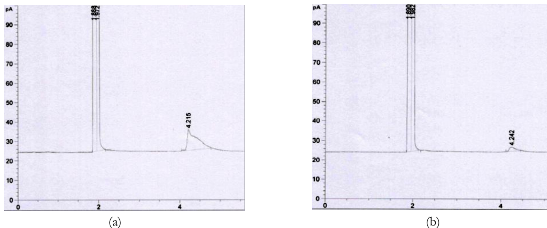
Figure 3. (a) chromatogram of analytical standard of Lambda-Cyhalothrin and (b) the amount of non-capsulated Lamda-Cyhalothrin
