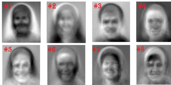
Figure (3) Eigenfaces
