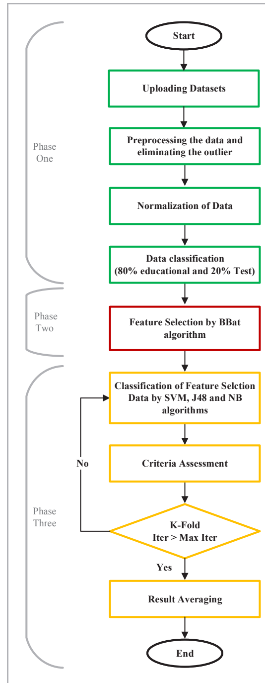
Figure 2: Three Phases of Proposed Method
