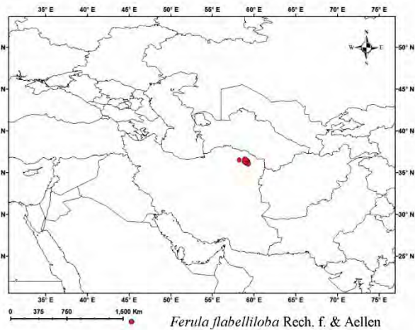
Fig. 8. Distribution maps of Merwia elements (arranged alphabetically as in table 1).
