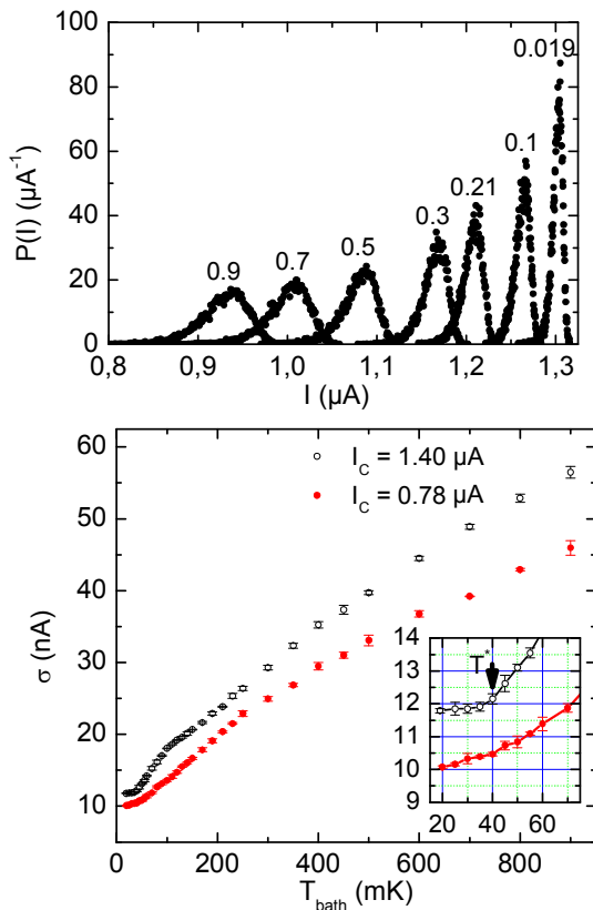
Figure 3. (color online) (a) Switching current probability distribution for different bath temperatures T_{\text{bath}} . The symbols represent data, and the lines are fits. (b) Temperature dependence of width \sigma for I_{c0}=1.40 \mu\text{A} and B=0 \text{ T} (open points) and I_{c0}=0.78 \mu\text{A} and B=2 \text{ mT} (full points). In the inset the low temperature part. (below 75 mK) is in evidence. Adapted from [11].
