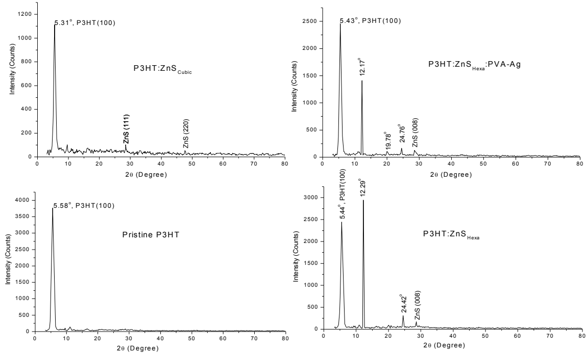
Figure 4. X-ray diffractogram of the samples.
