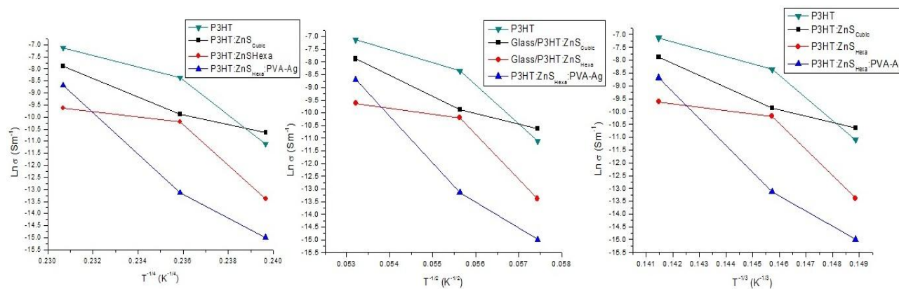
Figure 6. a) Lnσ vs. T -1/4 graph. b) Lnσ vs. T -1/2 graph. c) Lnσ vs. T -1/3 graph.
