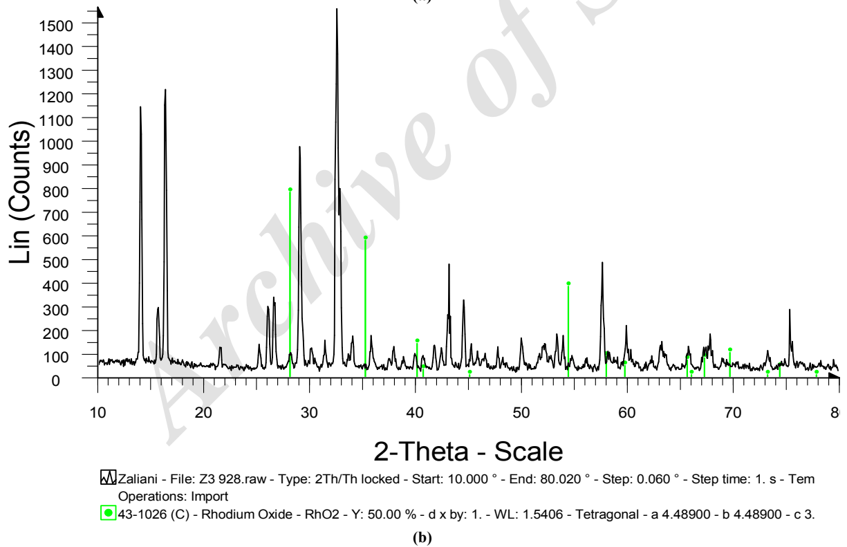
Figure 5. XRD pattern of KTP3 sample: a) to confirm the growth of \text{KTiPO}_4 crystal, b) to detect the existence of \text{RhO}_2 impurity.
